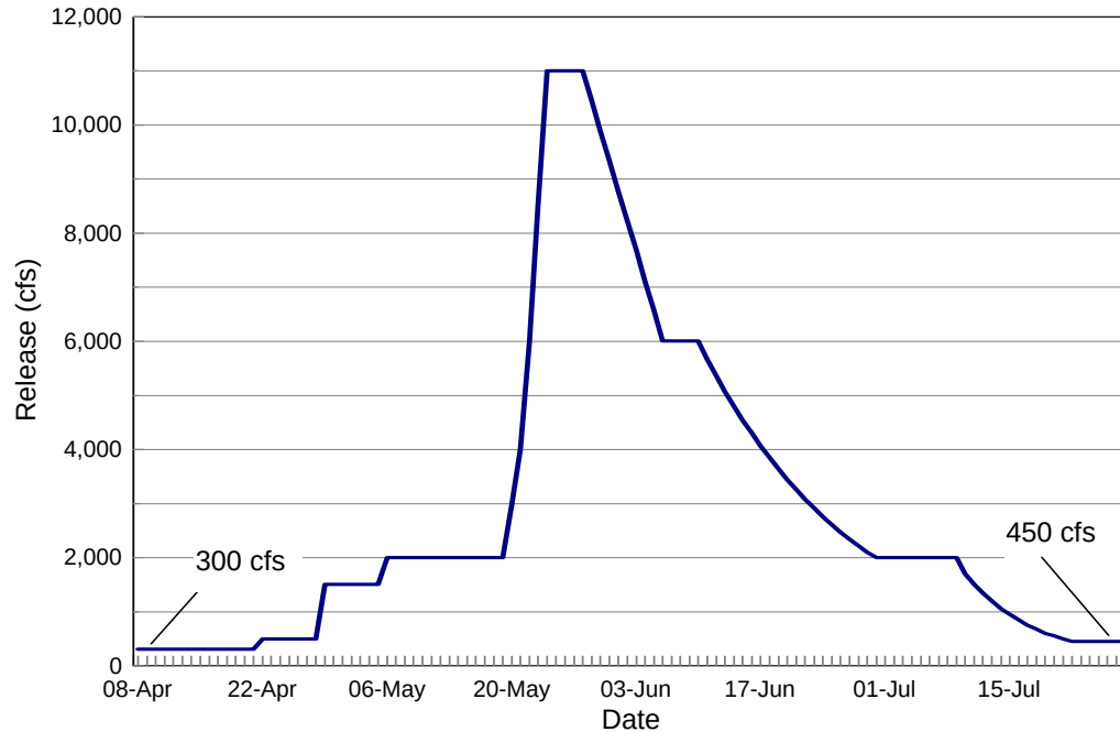
Figure 8.4. Recommended releases during an Extremely Wet water year. Releases are scheduled for 450 cfs from July 22 to October 15. Releases are scheduled for 300 cfs from October 16 to April 21.
