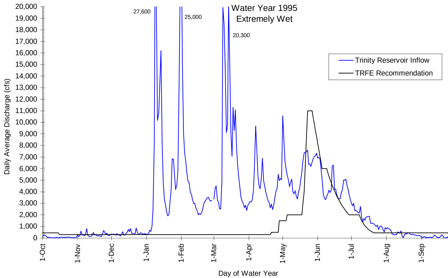
Figure 8.9. Recommended releases during an Extremely Wet water year compared to unimpaired inflow into Trinity Lake for WY 1995. Instantaneous peak discharges that exceeded the Y-axis maximum are indicated by values (cfs) placed next to the corresponding peak.
