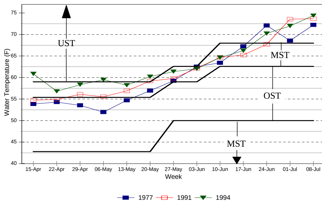
Figure K.3. Predicted water temperatures at Weitchpec (RM 0.0) during spring under the CRITICALLY DRY water year schedule. UST = Unsuitable Smolt Temperatures, MST = Marginal Smolt Temperatures, and OST = Optimal Smolt Temperatures.
